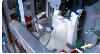
2 Bag opening
