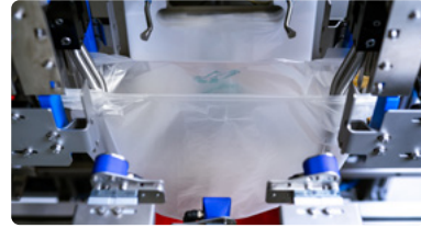
3 Bag spreading
