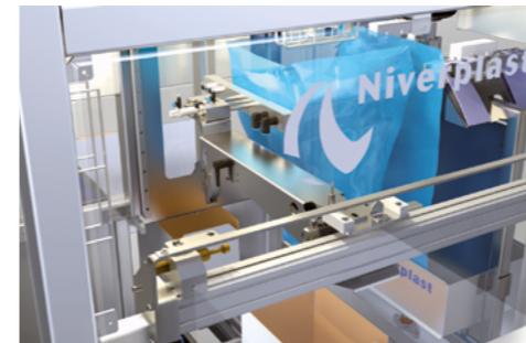
3 Bag opening
