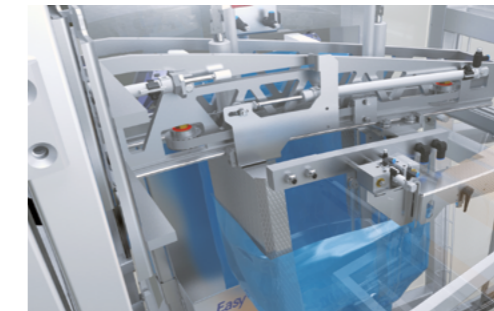
4 Bag spreading
